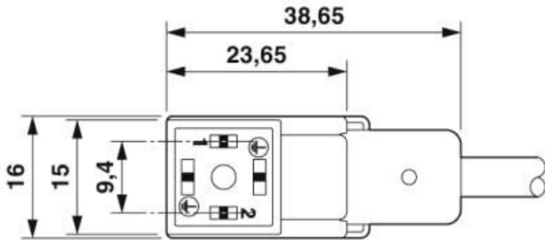
Valve connector, type CI
