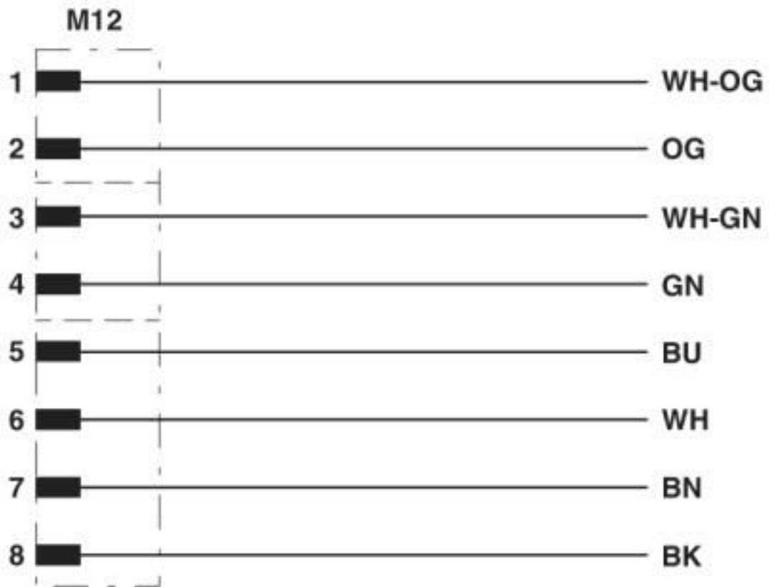
Circuit diagram
