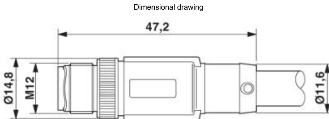
M12 connector, straight, shielded
