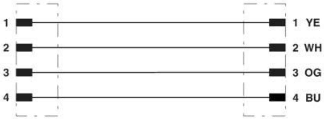
Contact assignment of M8 plugs
