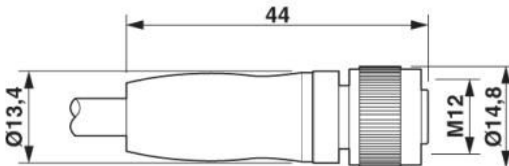
Dimensional drawing
