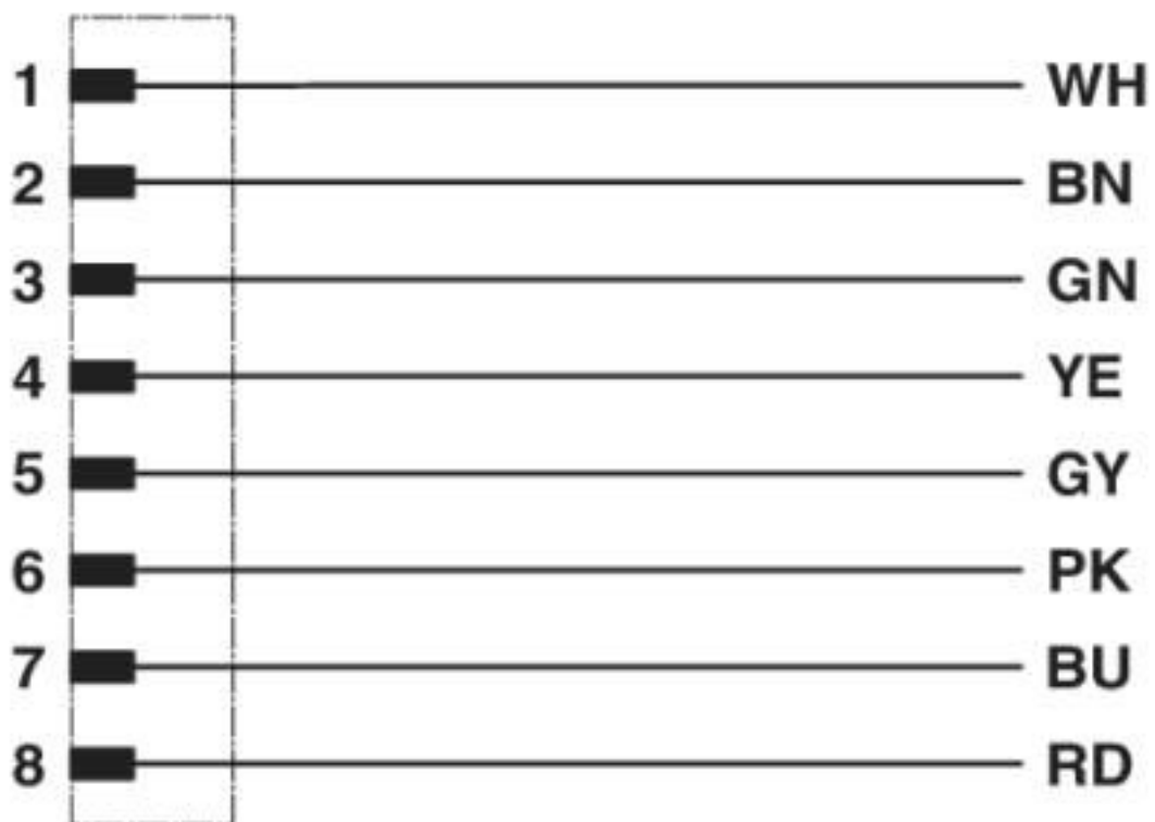
Contact assignment of the M8 plug
