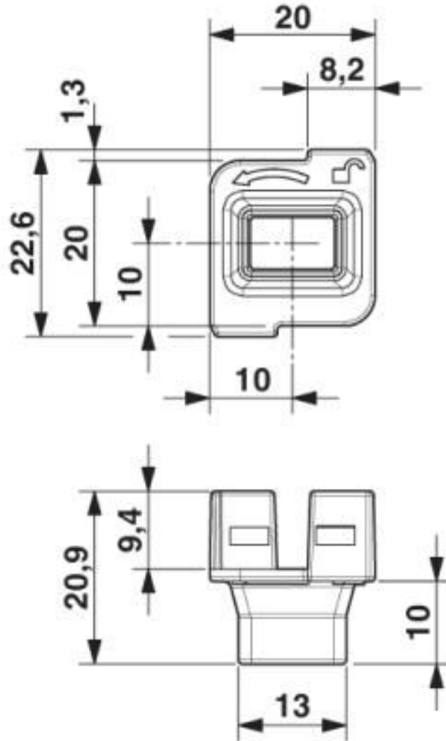
Dimensional drawing
