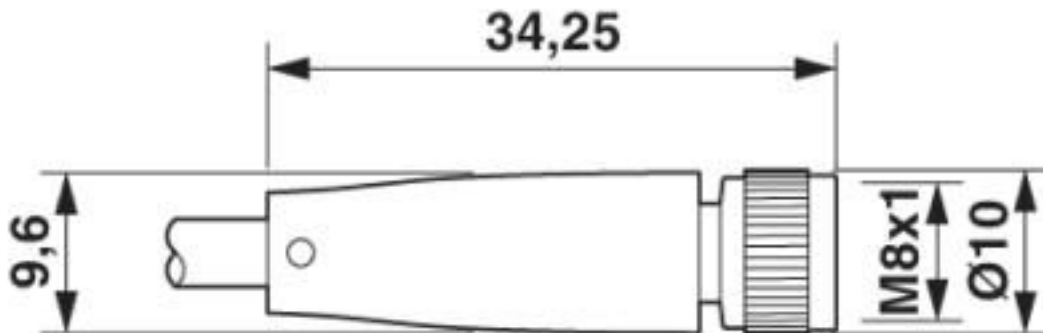
Dimensional drawing
