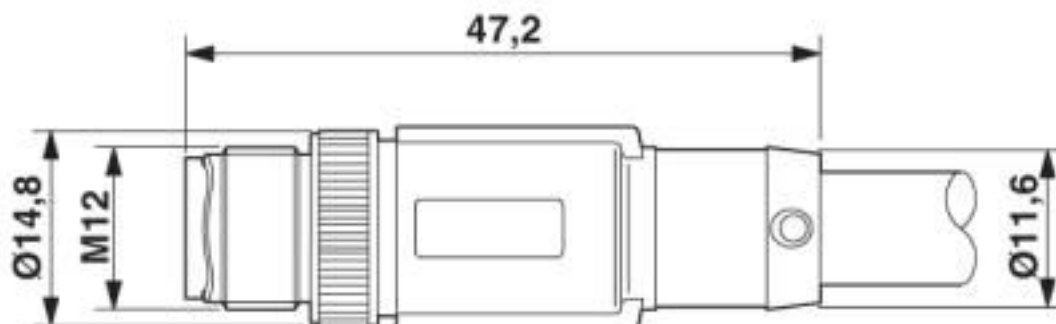
Plug, M12 x 1, straight, shielded
