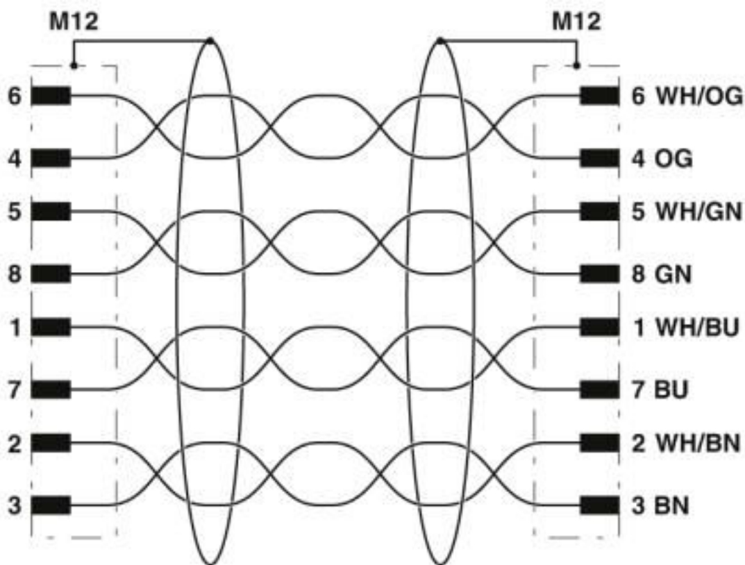
Circuit diagram
