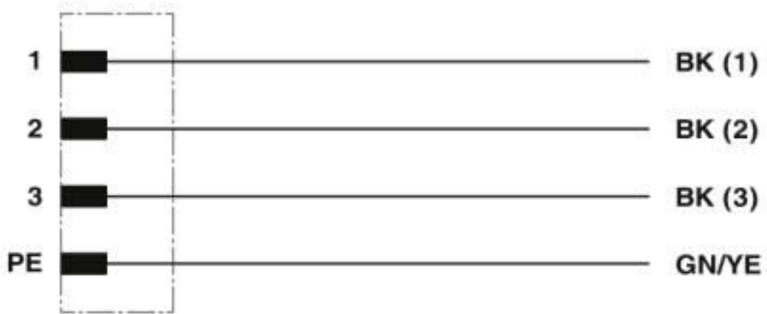
Circuit diagram
