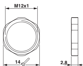
Dimensional drawing
