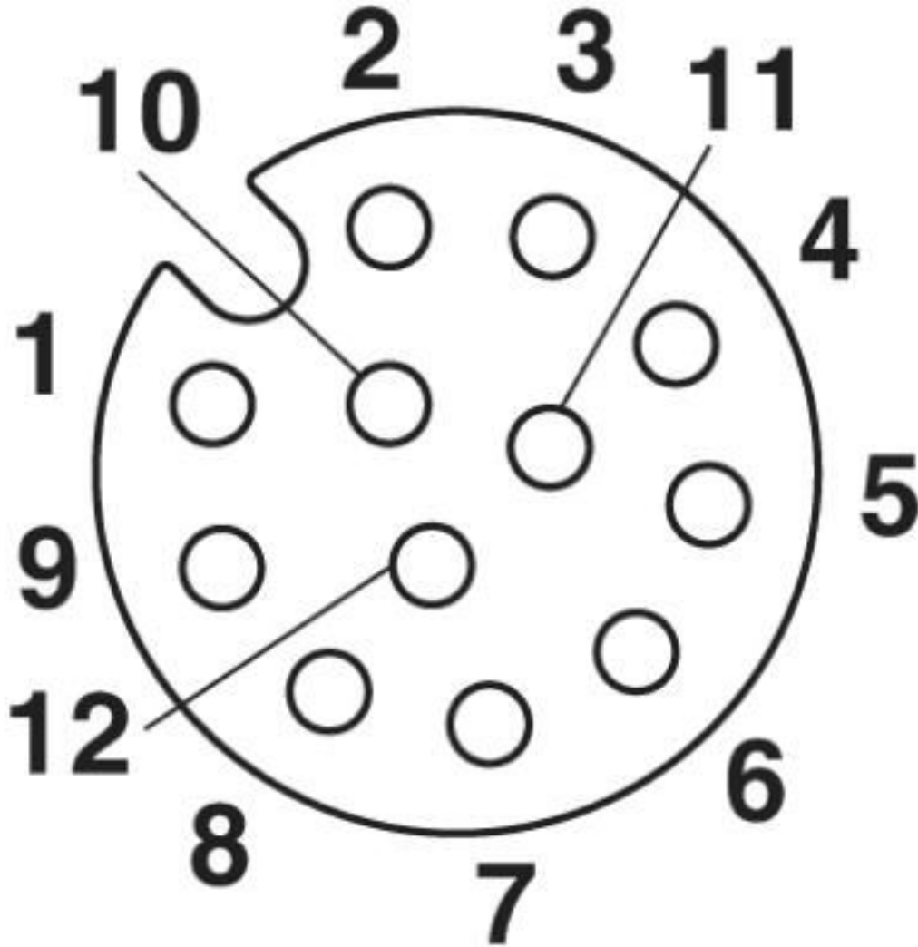
Pin assignment of M12 socket, 12-pos., A-coded, view of socket side, assignment: see connection drawing
