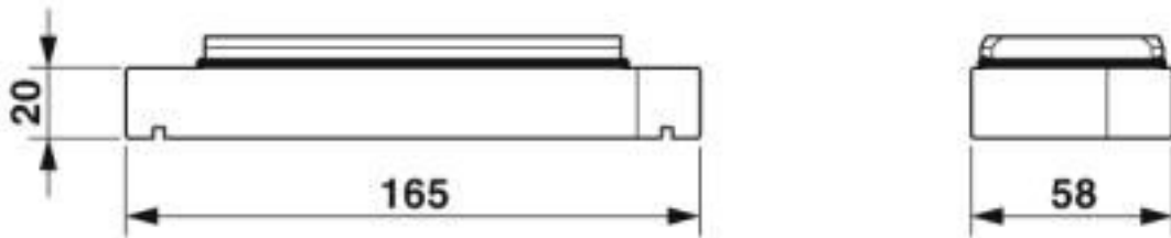
Dimensional drawing
