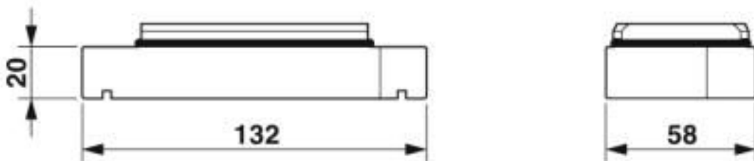
Dimensional drawing
