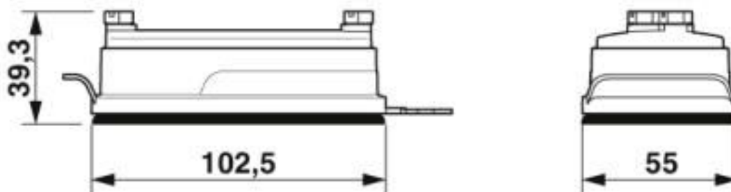
Dimensional drawing
