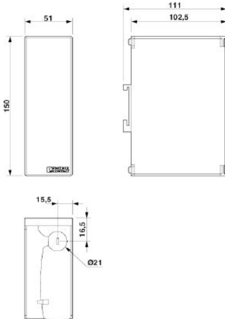
Dimensional drawing
