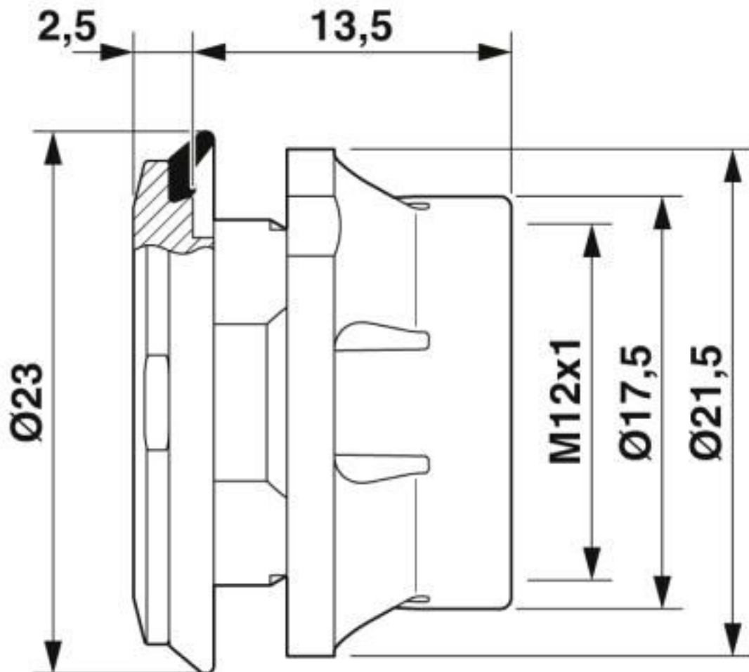
Dimensional drawing
