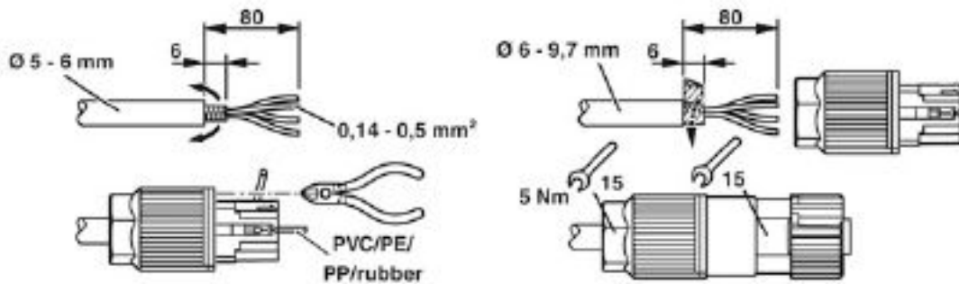
Functional drawing
