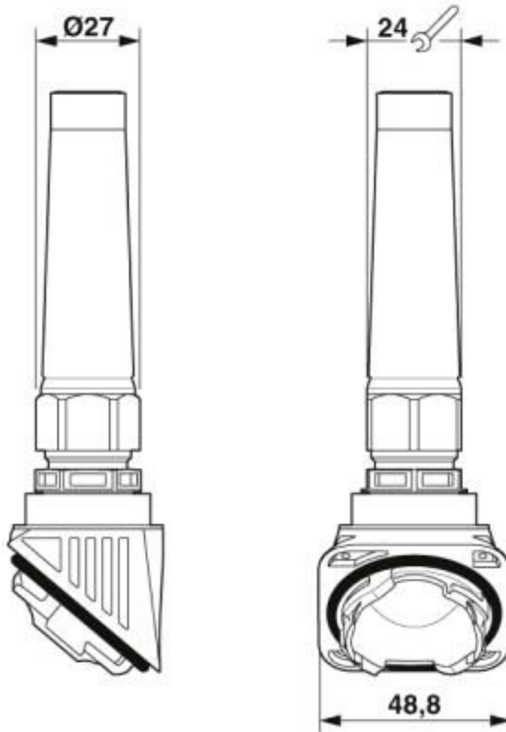
Dimensional drawing
