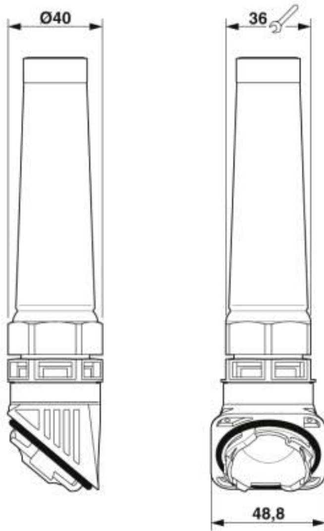
Dimensional drawing
