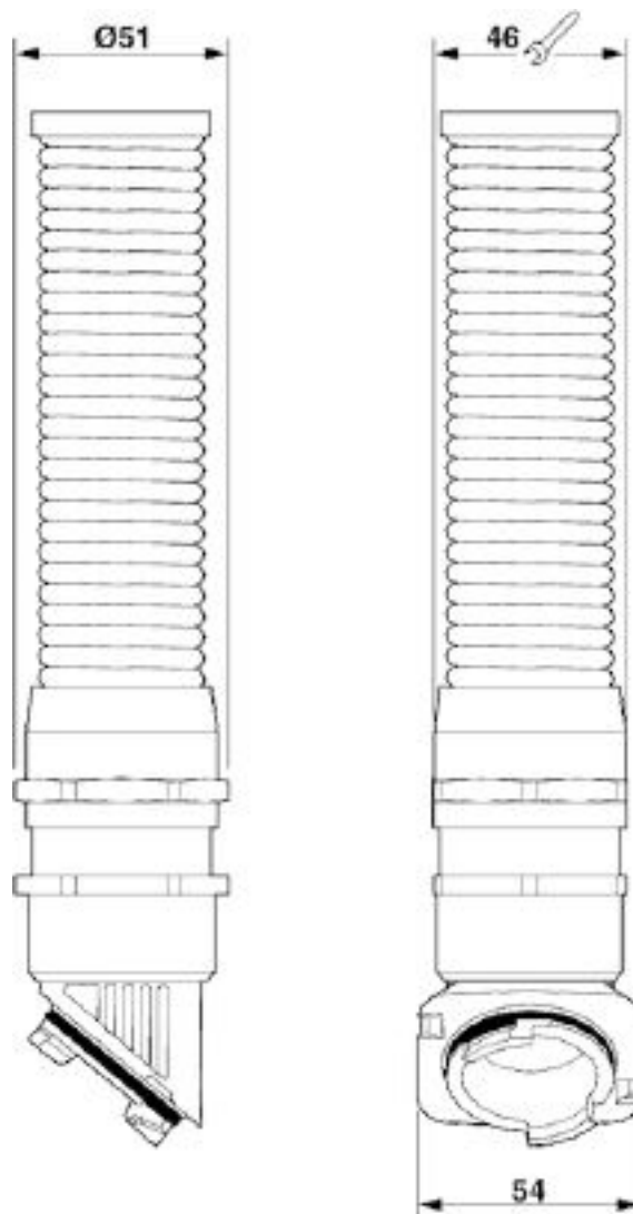
Dimensional drawing
