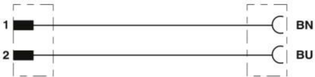
Contact assignment of the DEUTSCH connectors
