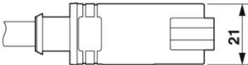
DEUTSCH DT04-3P, top view and side view
