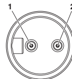
Plug pin assignment for 7/8"-16UNF plug, 5-pos.
