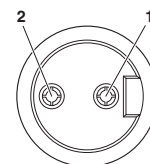
Pin assignment, socket, 7/8"-16UNF, 5-pos., view of female side
