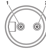
Plug pin assignment for 7/8"-16UNF plug, 5-pos.
