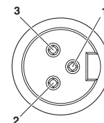
Pin assignment, socket, 7/8"-16UNF, 5-pos., view of female side
