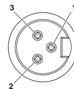
Pin assignment, socket, 7/8"-16UNF, 5-pos., view of female side
