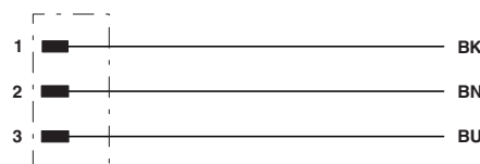
Contact assignment of the 7/8" connector and the 7/8" socket
