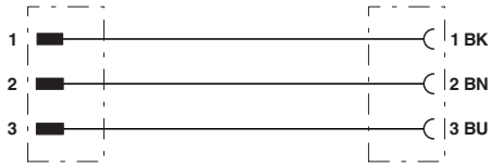
Contact assignment of the 7/8" connector and the 7/8" socket
