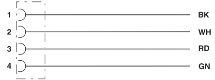
Contact assignment of 7/8" socket
