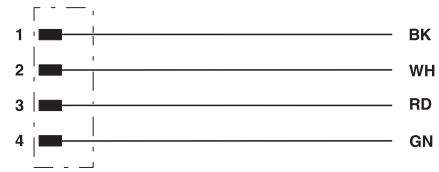
Contact assignment of the 7/8" connector and the 7/8" socket
