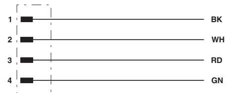
Contact assignment of the 7/8" connector and the 7/8" socket
