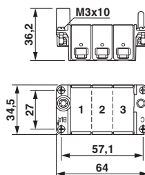
Dimensional drawing
