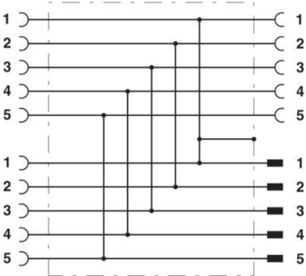
Contact assignment of the M12 H distributor
