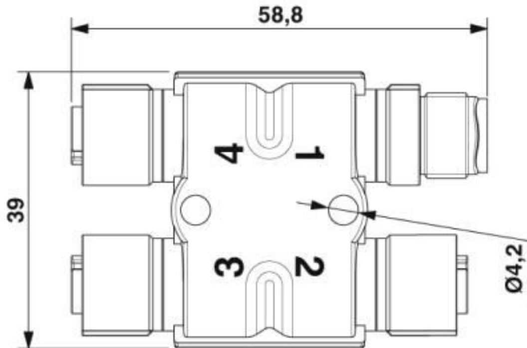
H distributor dimensional drawing
