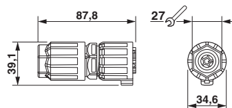
Dimensional drawing
