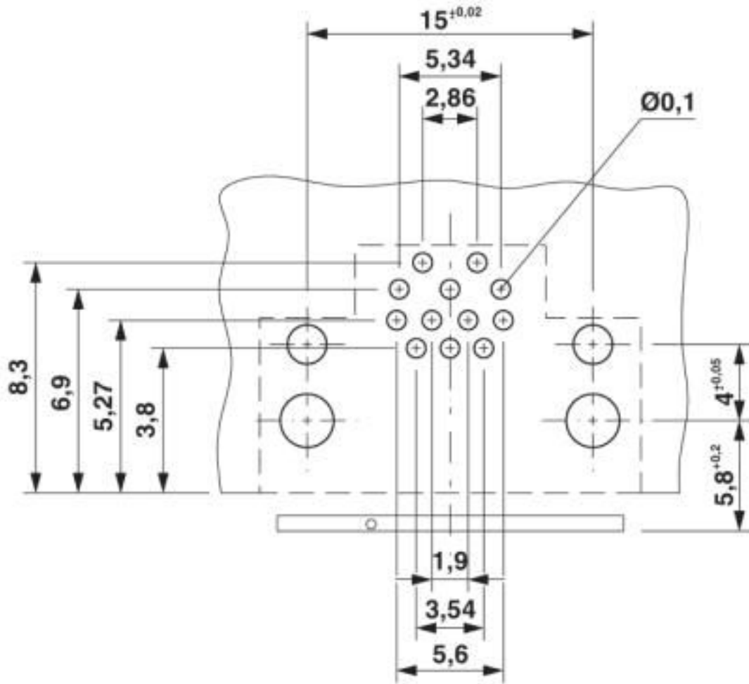
Drilling diagram
