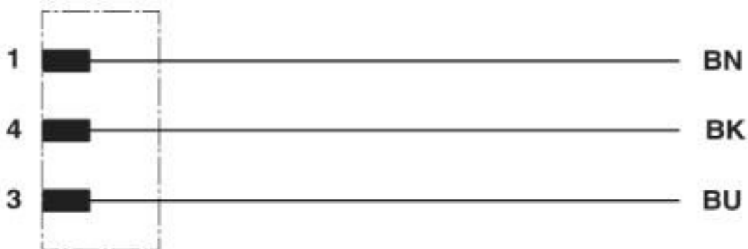
Contact assignment of the M12 plug
