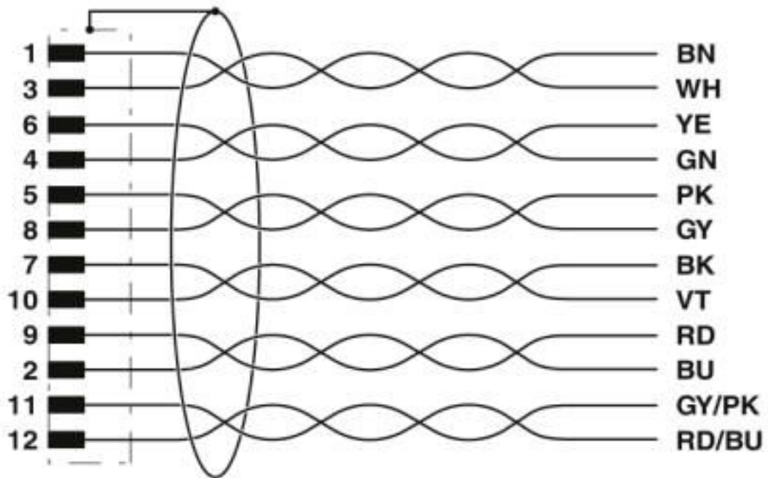
Circuit diagram
