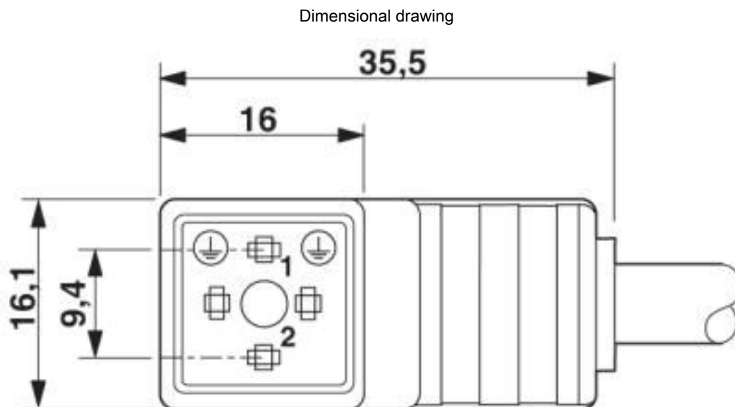
Valve connector, type CI
