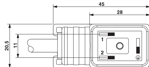
Valve connector, type BI
