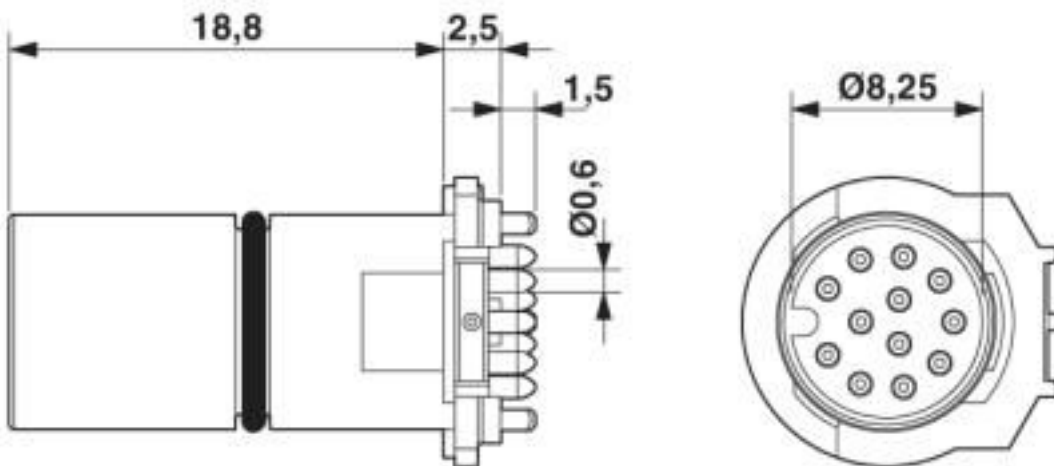
M12 flush-type connector
