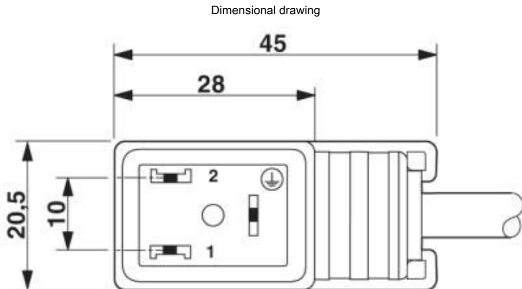
Valve connector, type B
