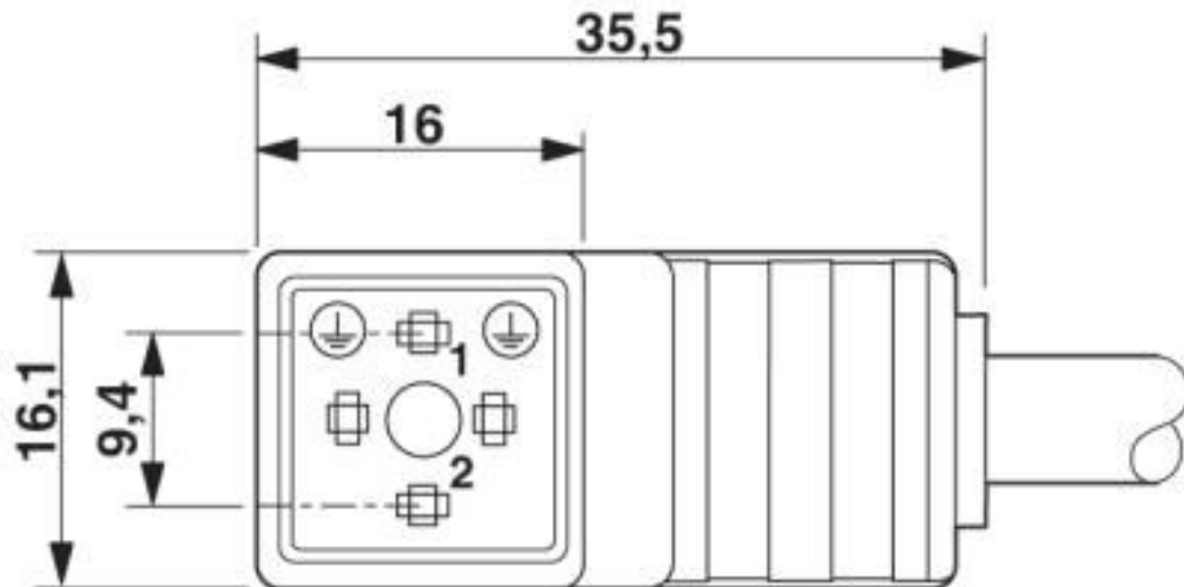
Valve connector, type CI
