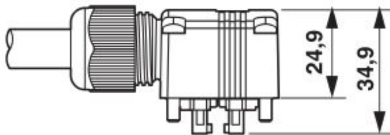
Dimensional drawing
