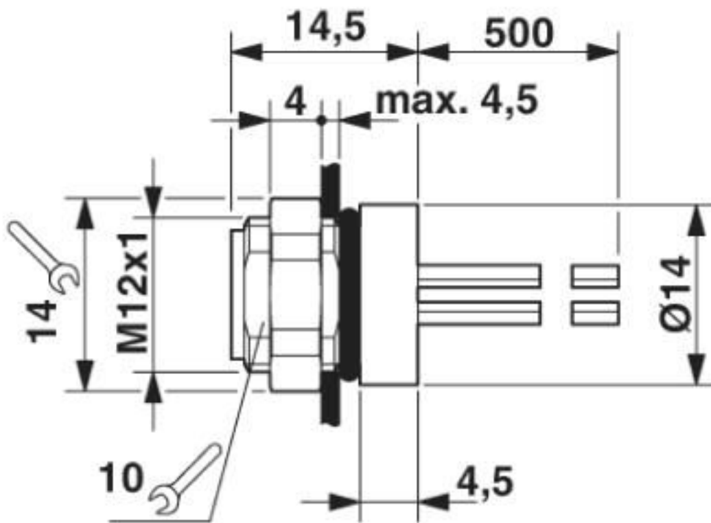
Dimensional drawing
