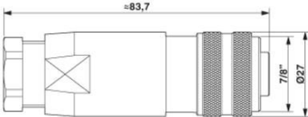
Dimensional drawing
