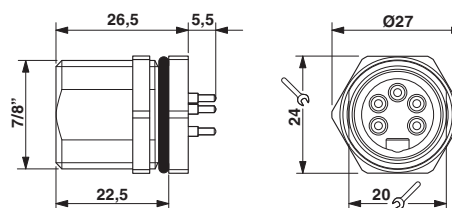
7/8" flush-type plug
