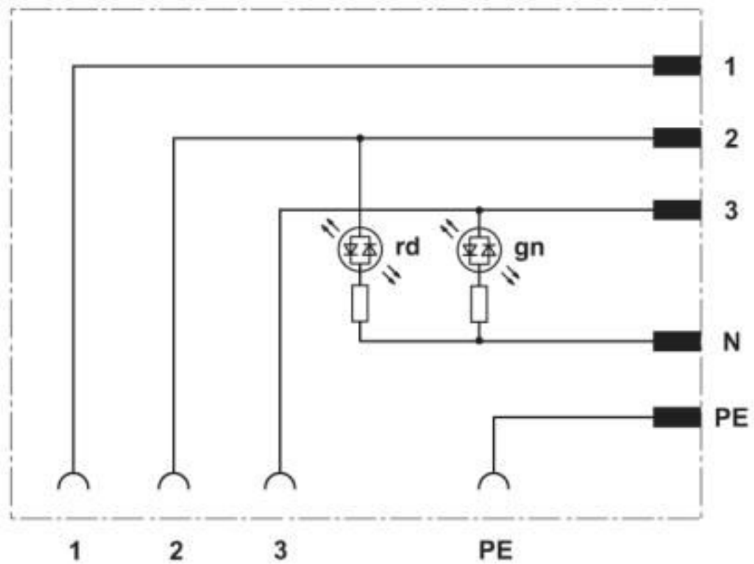
Circuit diagram
