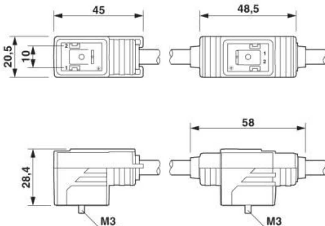
Double valve plug, 2 x type B
